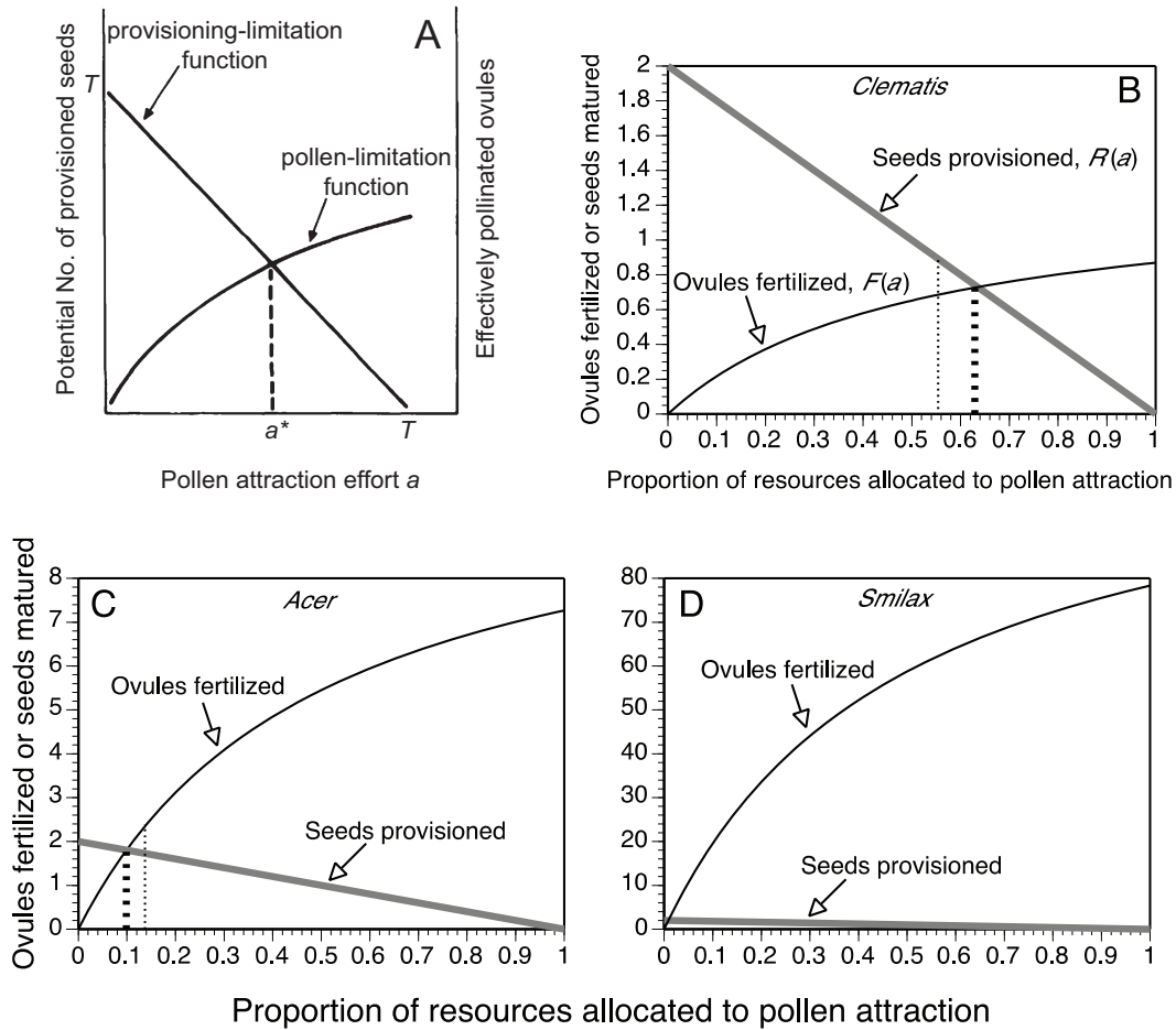
Figure 1: Influence of plant allocation to pollen attraction on the ability to secure ovule fertilizations and provision seeds for plant species with widely varying pre- and postpollination costs of seed production. A, Haig and Westoby’s (1988) original figure 1. Note that the maximum value of the pollen-limitation function is less than the maximum value of the provisioning-limitation function. Ovule-fertilization functions, F(a) , and seed-provisioning functions, R(a) , parameterized for Clematis micropphylla (B), a plant with high prepollination costs; Acer japonicum (C), a plant whose prepollination costs were near the median value; and Smilax glycyphylla (D), a plant with low prepollination costs. The optimal allocation to pollen attraction in a deterministic environment (thick dotted line) occurs where the two functions intersect. The optimal allocation in a stochastic environment (thin dotted line) includes an overinvestment in the less expensive component of reproductive effort. Changes in the functions describing the costs of ovule fertilization and seed maturation alter the predictions for optimal allocations to pollen attraction and the resulting importance of pollen limitation.
