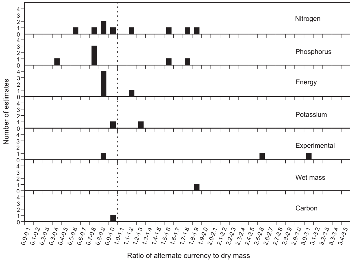
Figure 2: Influence of different measurement currencies (nitrogen, phosphorus, potassium, carbon, or energy content; wet mass; or use of experimental methods) on estimates of the proportional contribution of prepollination costs to the total costs (prepollination plus post-pollination) of seed production. Shown are the ratios of cost estimates relative to the estimate based on dry weight; a ratio of 1.0 indicates perfect agreement between an alternate currency and dry weight, whereas ratios >1.0 (or <1.0) indicate that alternate currencies support a larger (or smaller) proportional contribution of prepollination costs to the total costs of seed production. Estimates derived from a survey of the published literature (see app. H, available online, for a list of the taxa and literature citations).
